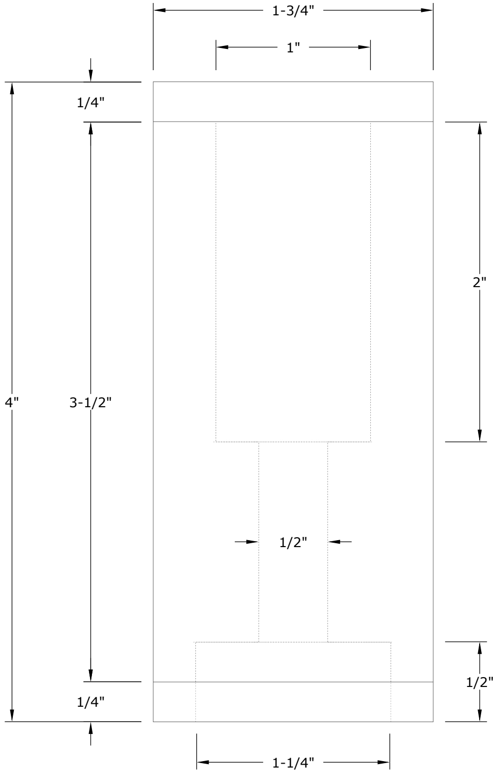
PROFILE VIEW 1-3/4" SQUARE
